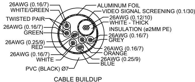
SECTION Z-Z
