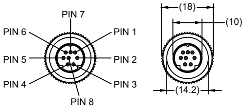
VIEW B
