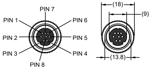
VIEW A
