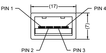
VIEW C
