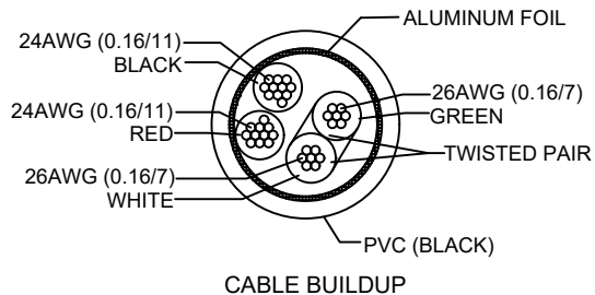
SECTION Y-Y
